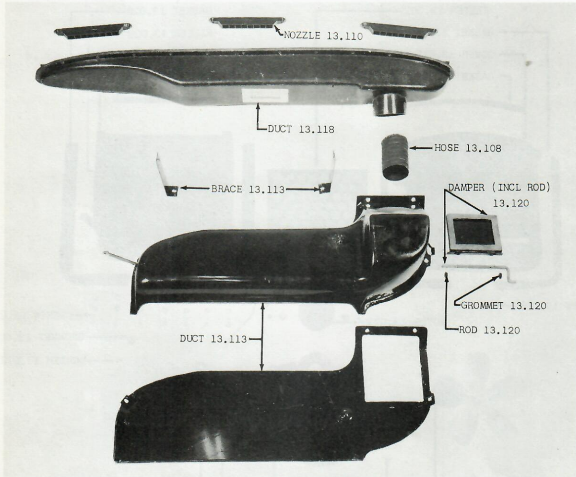
GROUP 13 - FIG. 2 - HEAT DISTRIBUTION DUCT 10-20-80 (LAC)
