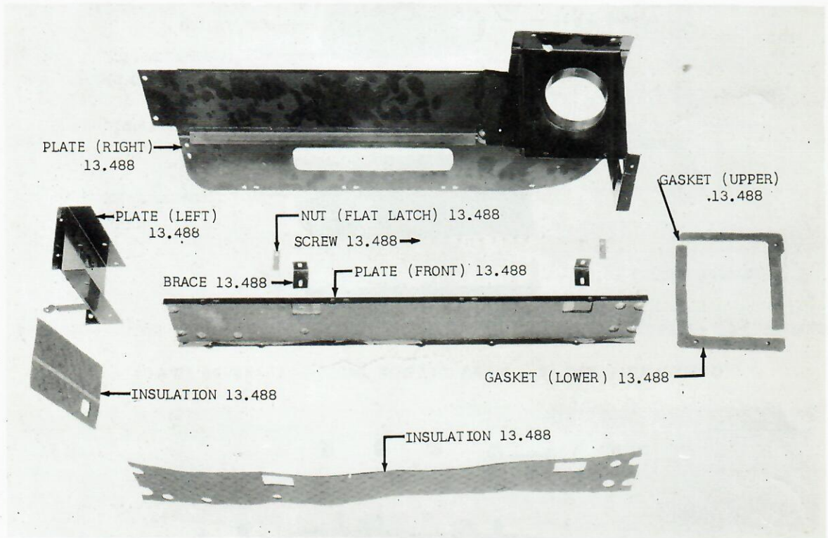
GROUP 13 - FIG. 3 - EVAPORATOR HOUSING PLATE 10-20-80 (WAC)
