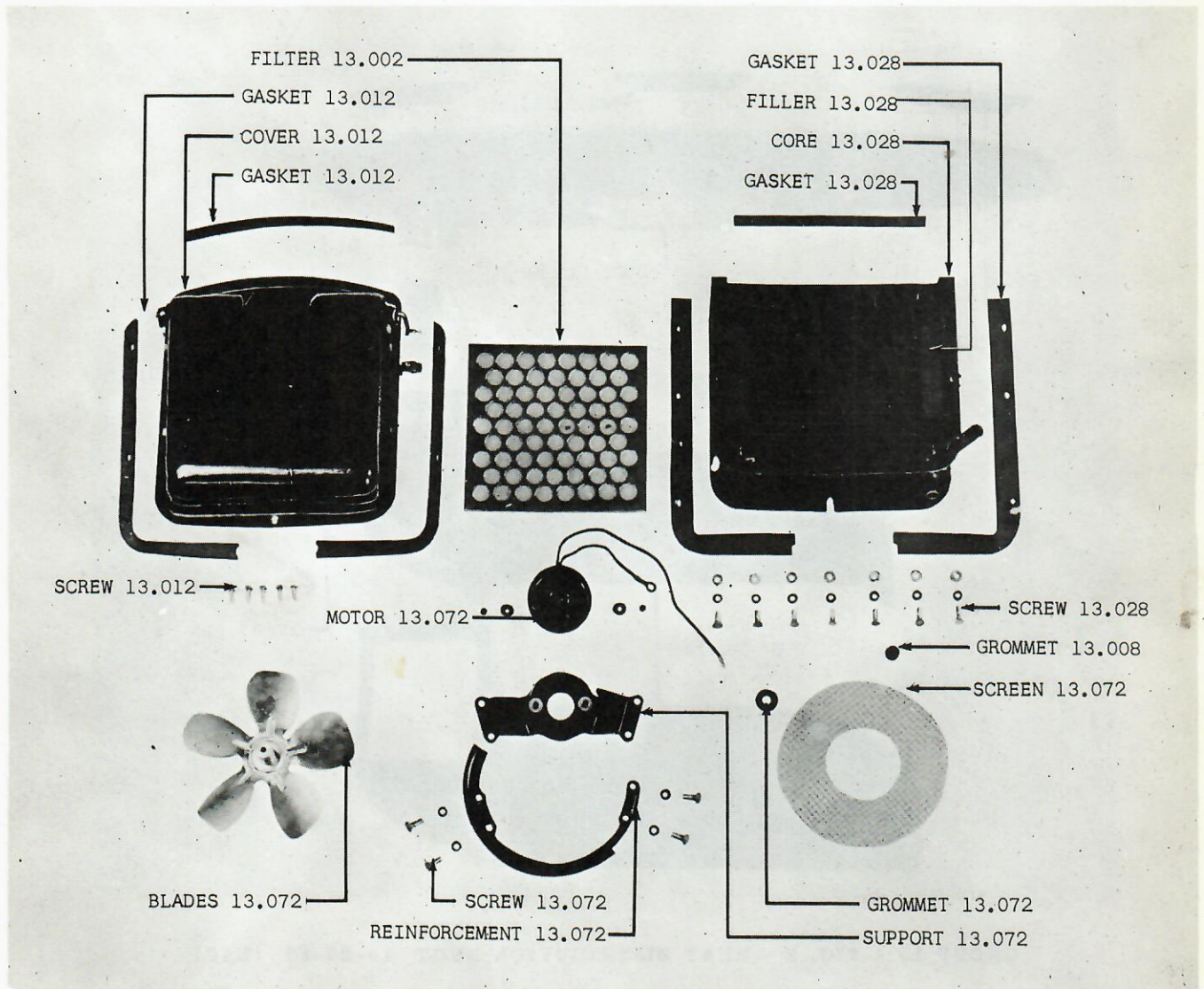
GROUP 13 - FIG. 1 - WEATHEREYE ASSEMBLY 01
