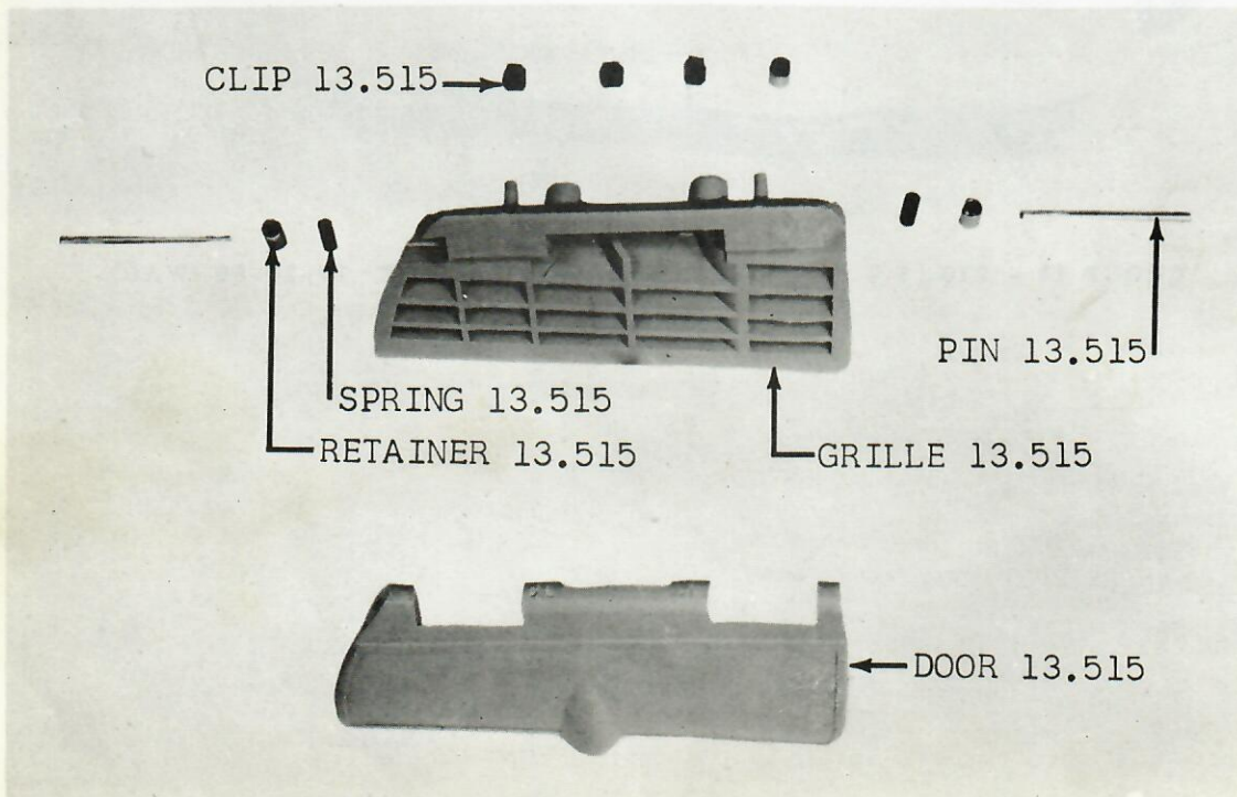
GROUP 13 - FIG. 5 - AIR CONDITIONING AIR DISCHARGE GRILLE 10-20-80 (WAC)
